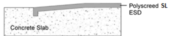
Termination Detail
