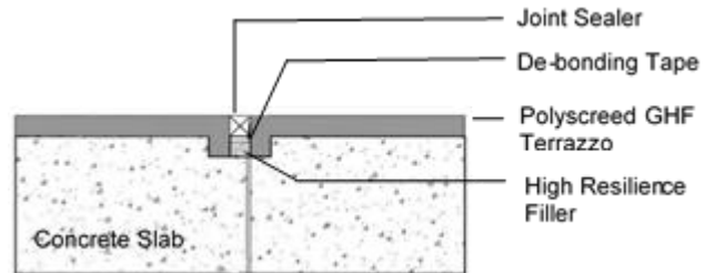
Termination Detail
