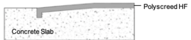
Termination Detail
